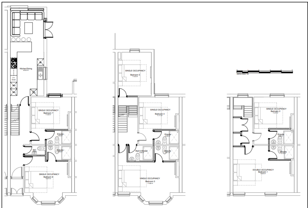
Figure 1 Proposed Floorplans
